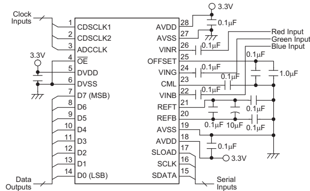
28-pin SSOP CDS Application Circuit
