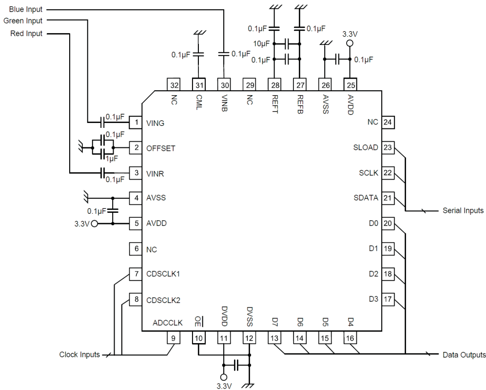
32-pin QFN CDS Application Circuit
