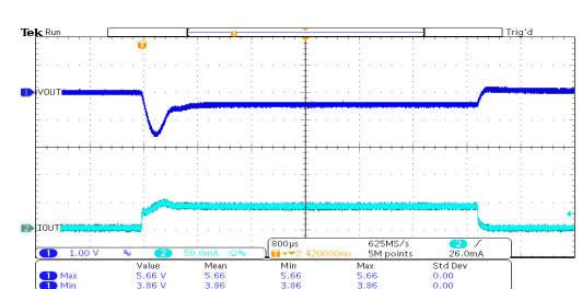
Load Transient Response: HT7550-3 ( V_{IN}=7V , I_{OUT}=0mA \sim 40mA )
