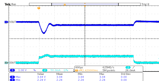
Load Transient Response: HT7533-3 ( V_{IN}=5.3V , I_{OUT}=0mA \sim 40mA )
