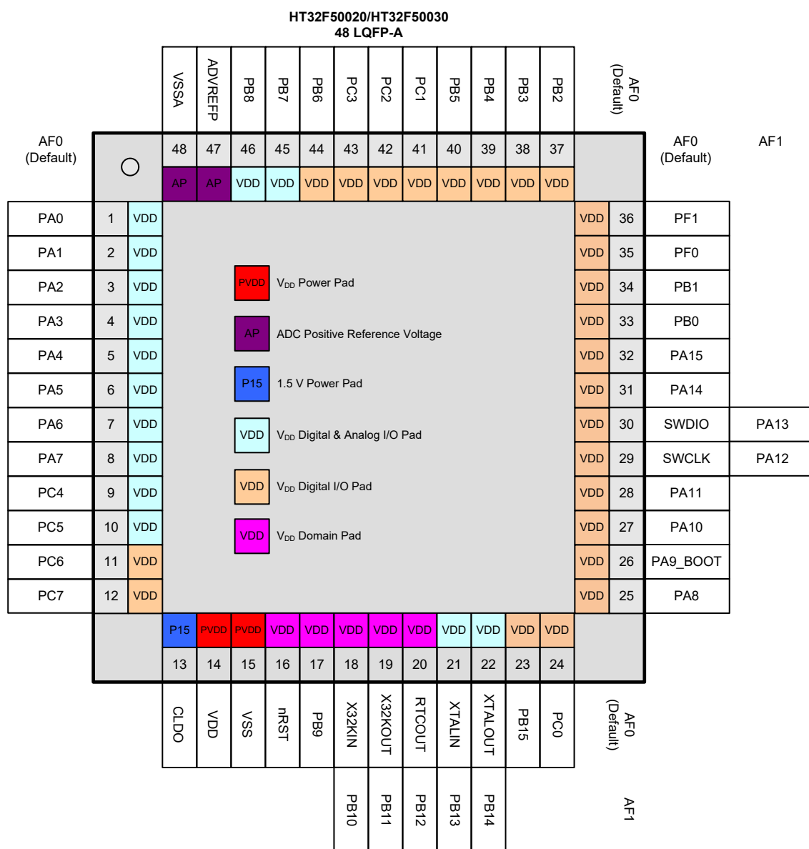
Figure 8. 48-pin LQFP Pin Assignment
