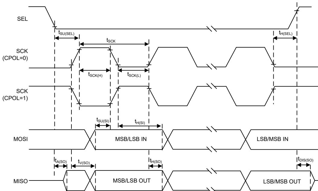
Figure 12. SPI Timing Diagram – SPI Slave Mode with CPHA = 1
