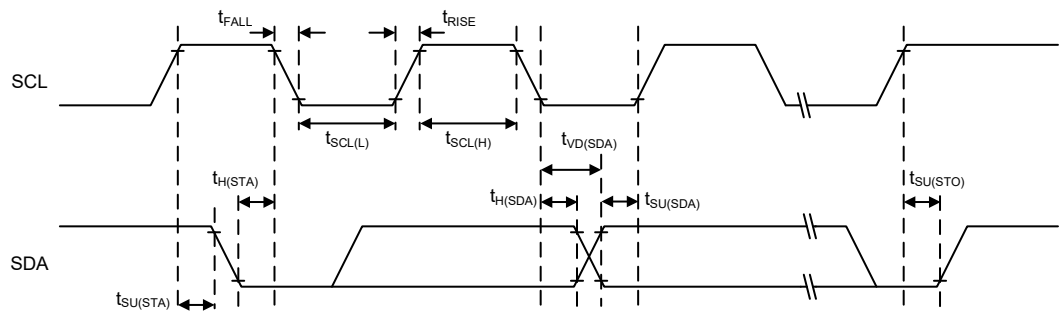
Figure 10. I 2 C Timing Diagram
