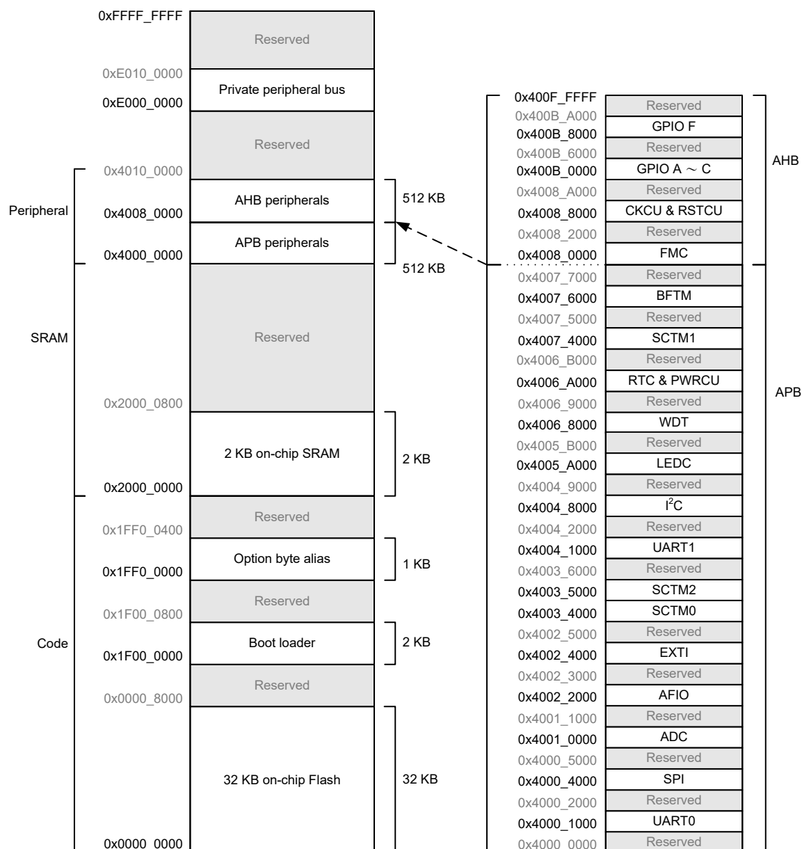
Figure 2. Memory Map
