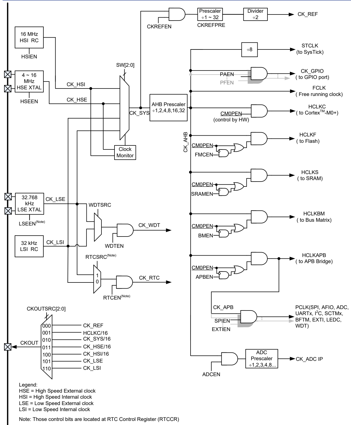
Figure 3. Clock Structure
