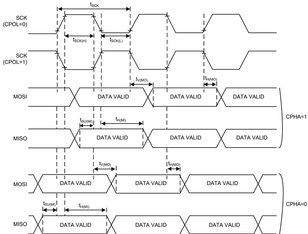
Figure 11. SPI Timing Diagram – SPI Master Mode
