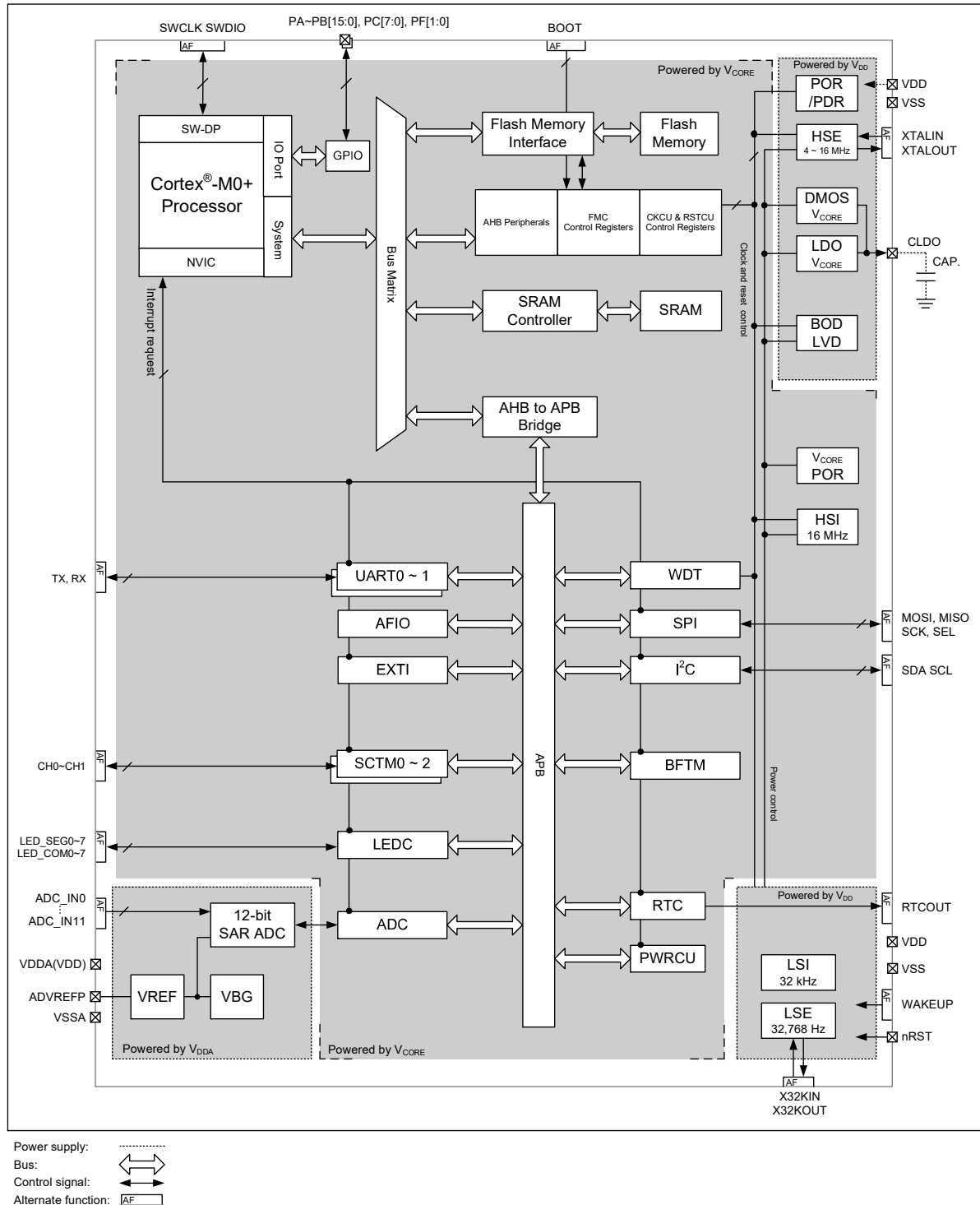
Figure 1. Block Diagram
