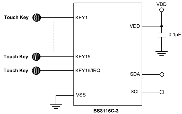
BS8116C-3 (24-pin SSOP)
