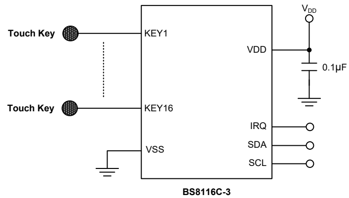
BS8116C-3 (24-pin SSOP)
