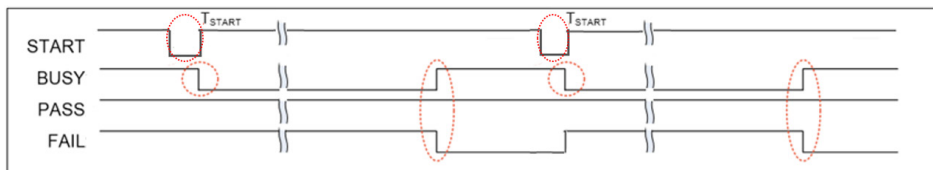
Failed Programming Waveform
