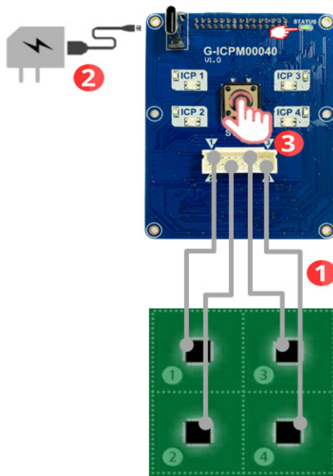
Offline Programming – Single Module
