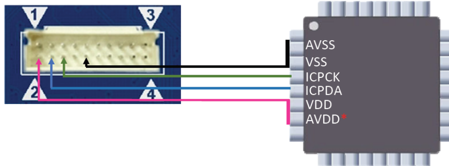
20PIN PHB Connector (32-Bit MCU Program)
