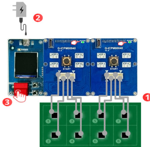
Offline Programming – Module & Base Board
