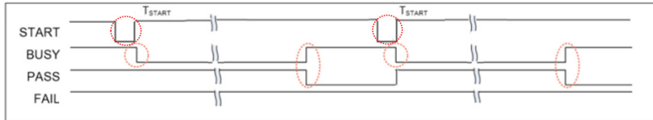
Successful Programming Waveform
