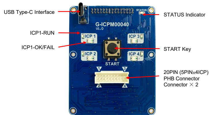
G-ICPM00040 – Programming Module
