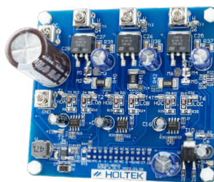
MVPB 17 ~ 60 V / 20 A
