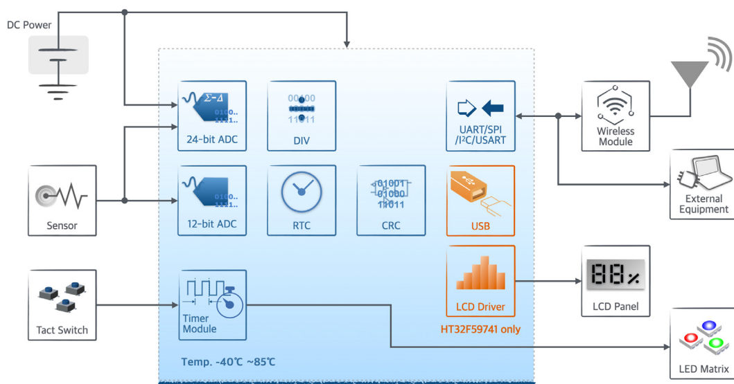
HT32F59041/741 Arm® Cortex®-M0+
